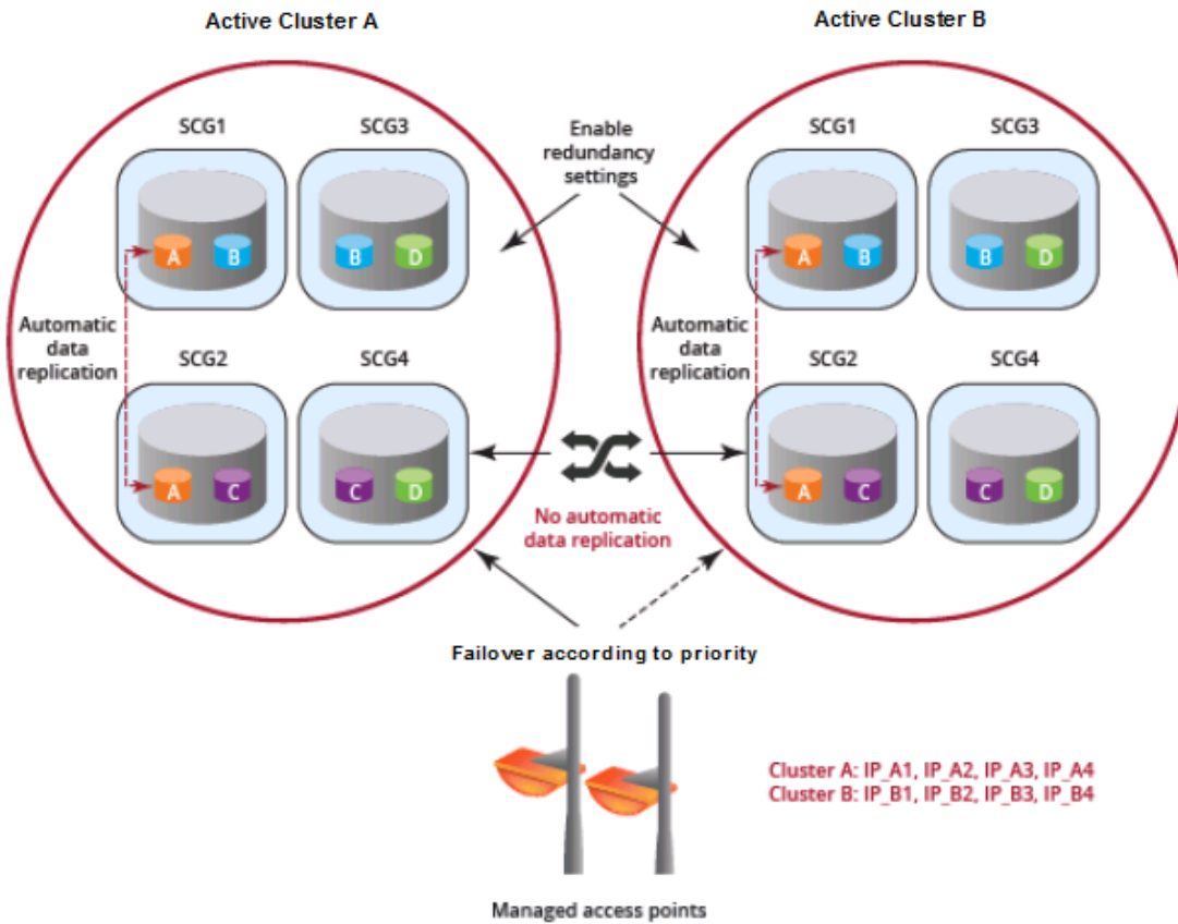
FIGURE 64 Cluster Redundancy for Active-Active Mode
