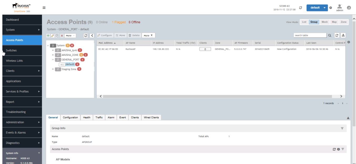
FIGURE 44 Access Point
