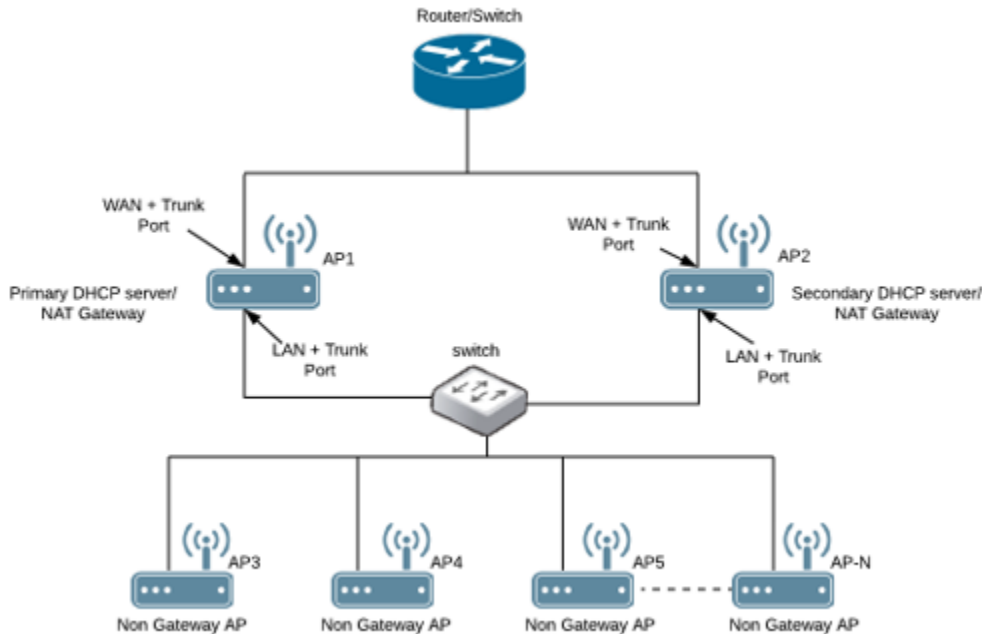
FIGURE 218 Hierarchical AP Topology
