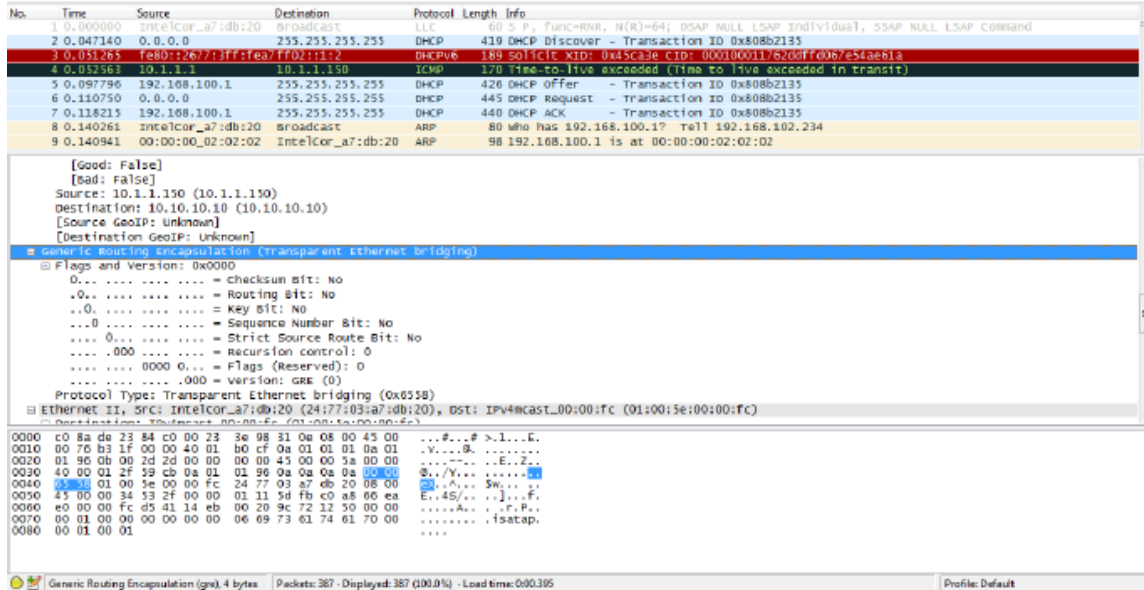
FIGURE 281 Example of SoftGRE packet format
