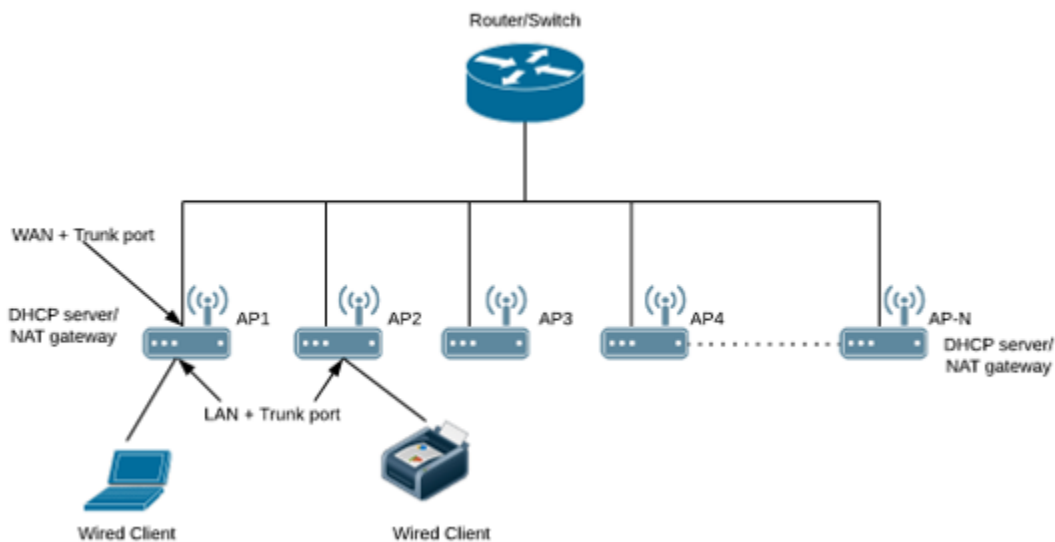
FIGURE 216 Single AP Topology
